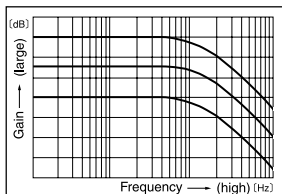
Fig. 4 Frequency response with current feedback (Response remains uniform even when gain changes)
